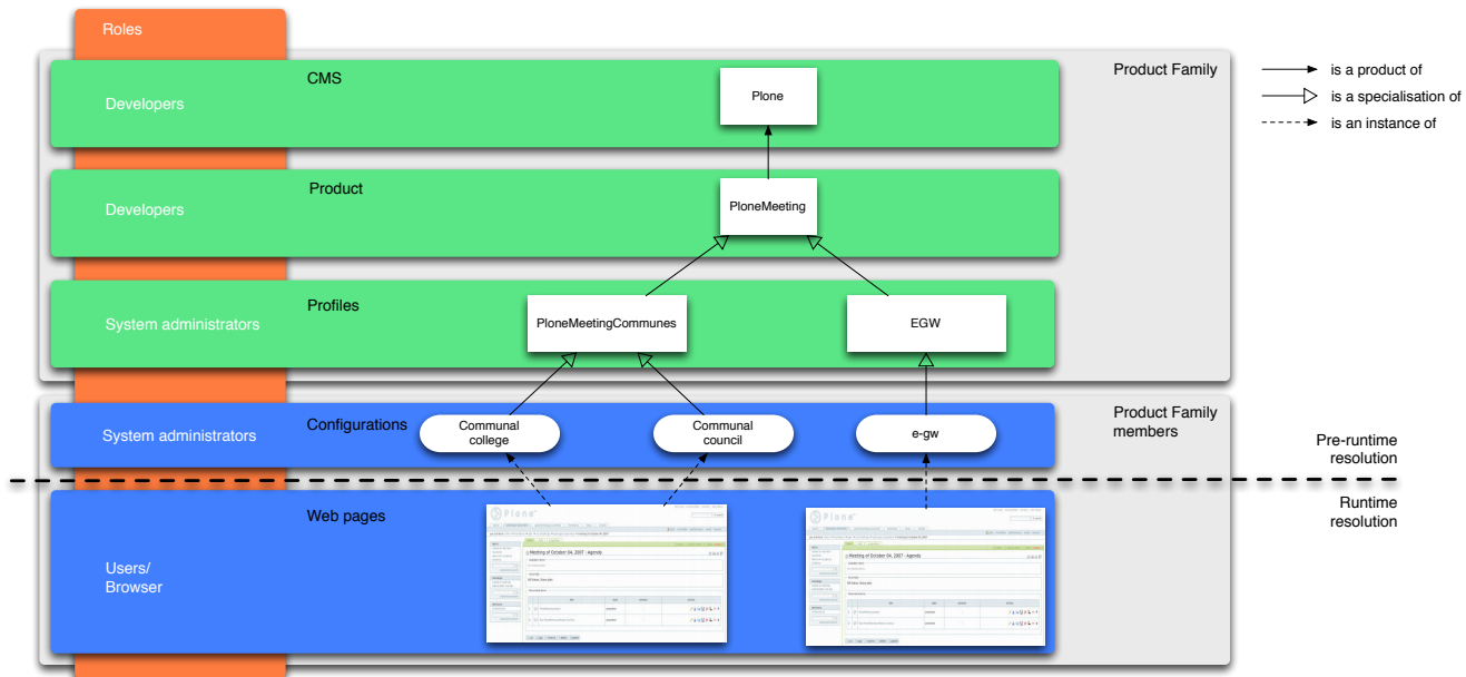
Figure 1. Overview of PloneMeeting variability resolution levels
