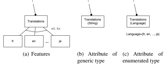
Figure 6. Modelling many subfeatures in FDs
