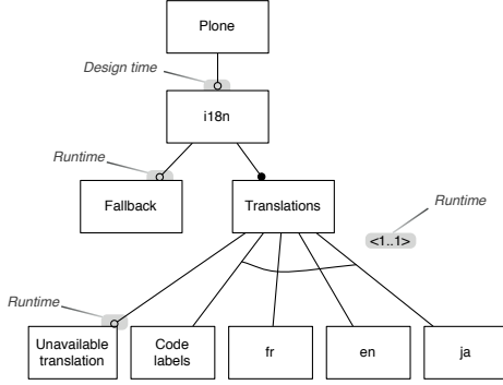
Figure 4. Plone i18n FD: design and runtime together
