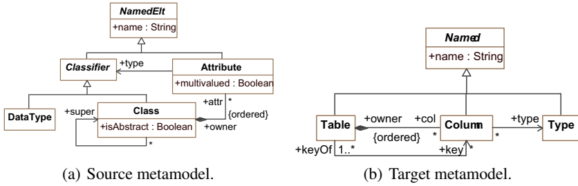
Fig. 1. Transformation metamodels
