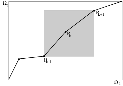
Figure 6. Proportional mutation.
