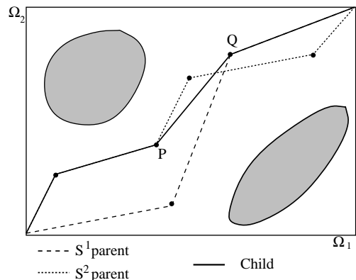
Figure 4. Crossover operator.
