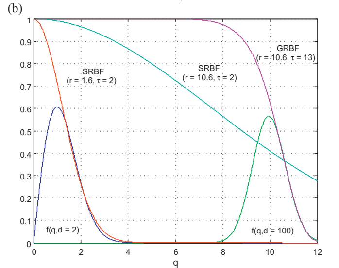
Fig. 3. Probability density of a point from a normal distribution to be at distance q .
